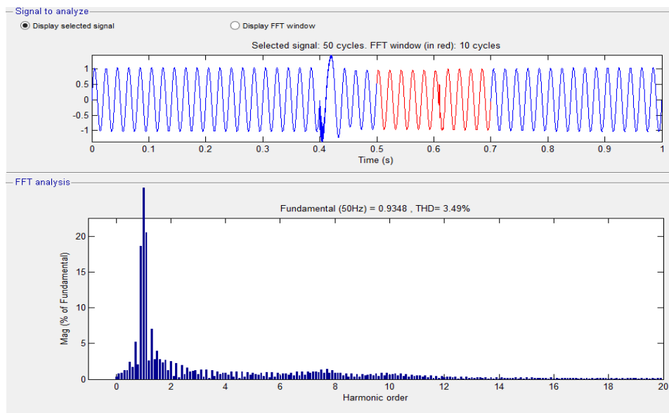
Figure 11 THD analysis of DVR
