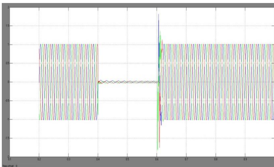
Fig.-7 Source Voltage waveform during Fault with Uncompensated system
