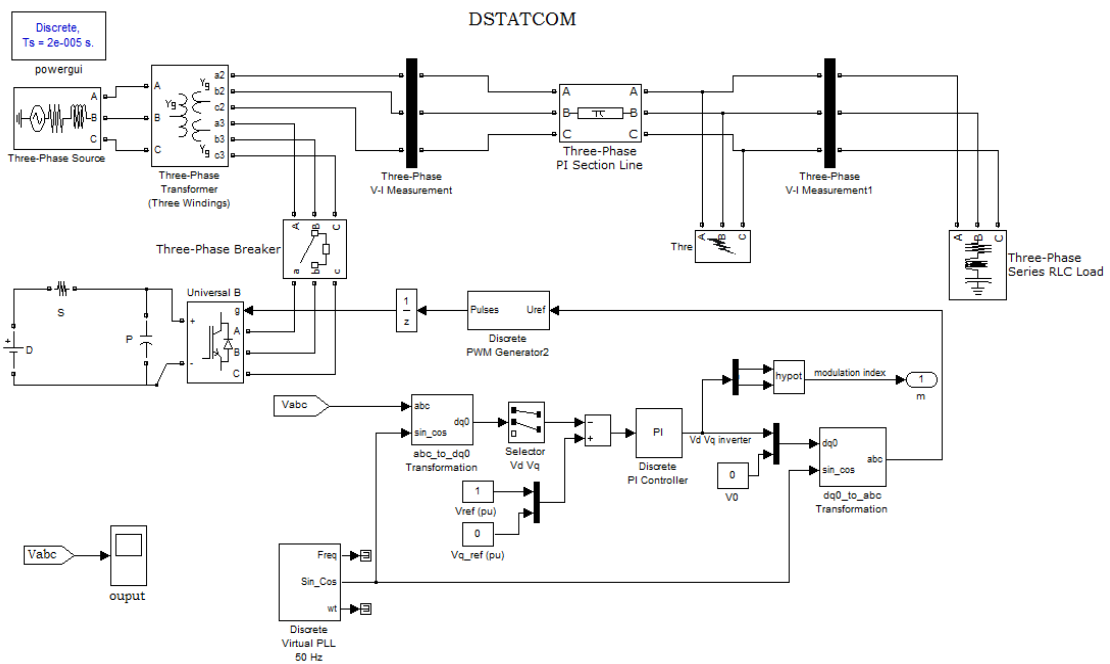
Figure 6 MATLAB model of DSTATCOM connected system
