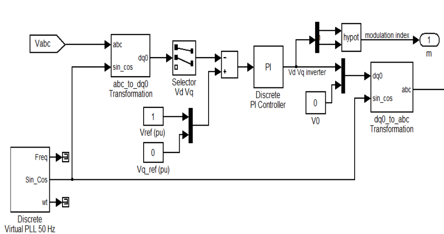
Figure 1 Schematic diagrams of control block.
