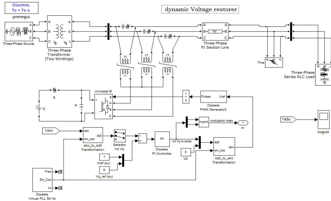
Figure 5 MATLAB model of DVR connected system
