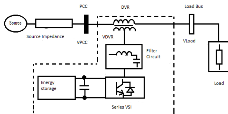
Figure 2 DVR series connected topology
