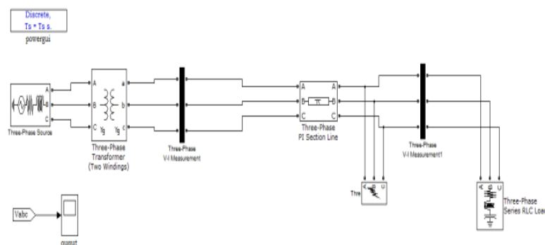
Figure 4 MATLAB model of DSTATCOM connected system
