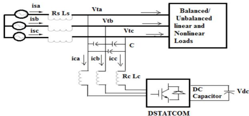
Fig-3: Schematic Diagram of DSTATCOM
