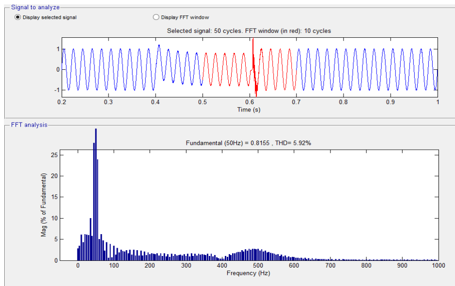
Figure 10 THD analysis of DSTATCOM
